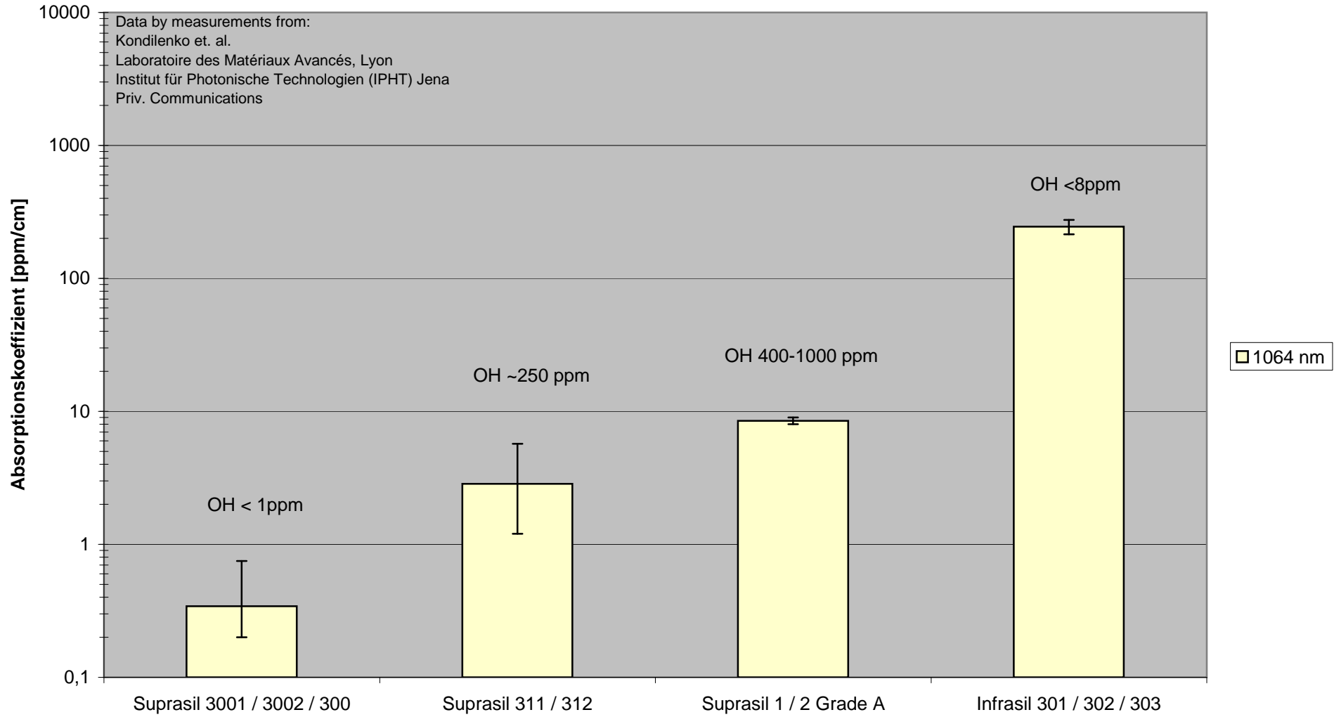
Typical Absorption of different Heraeus Material Grades @ Wavelength = 1064nm
